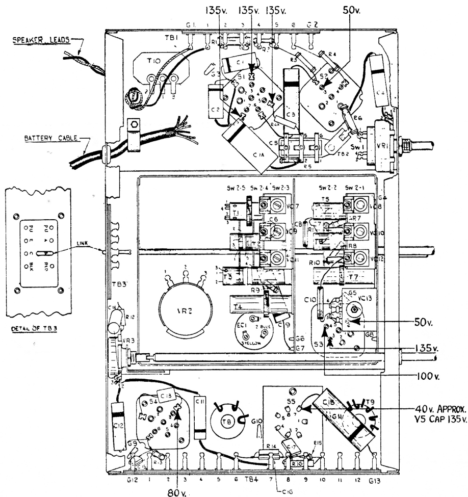
UNDER CHASSIS DIAGRAM.
